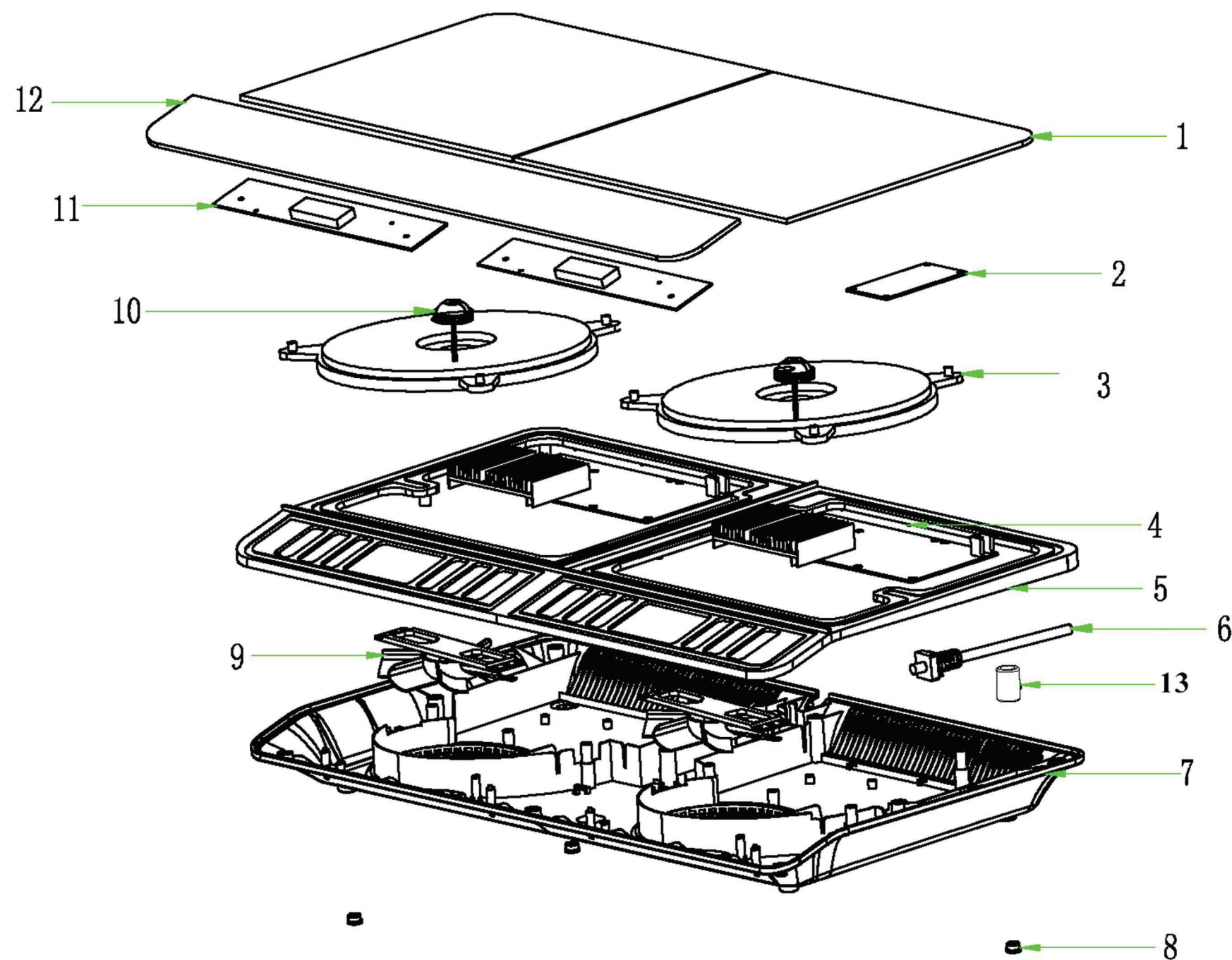
IC-3500D induction cooker
